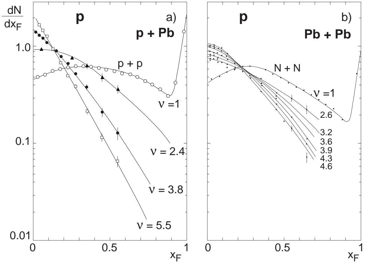
Figure 6: x_F distributions of net proton ( p-\bar{p} ) distributions for a) p+p and p+Pb collisions of different centrality ( \nu is the mean number of projectile collisions; yields in p+Pb are corrected for target feed-over using \pi +Pb data) and for b) N+N and Pb+Pb collisions of different centrality ( \nu is the mean number of collisions of each participating nucleon; yields are normalized by the number of participant pairs for each centrality bin; the N+N distribution was obtained from p+p \rightarrow p+X and p+p \rightarrow n+X data using the proper p/n ratio for the Pb nucleus).
