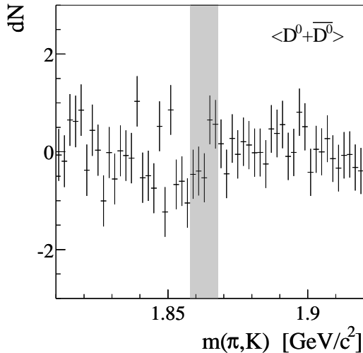
Figure 3: Invariant mass spectrum in the D^0 , \bar{D}^0 mass region, scaled to the absolute average yield per event. The background has been subtracted by fitting a parabola to the bands outside the shadowed area.
