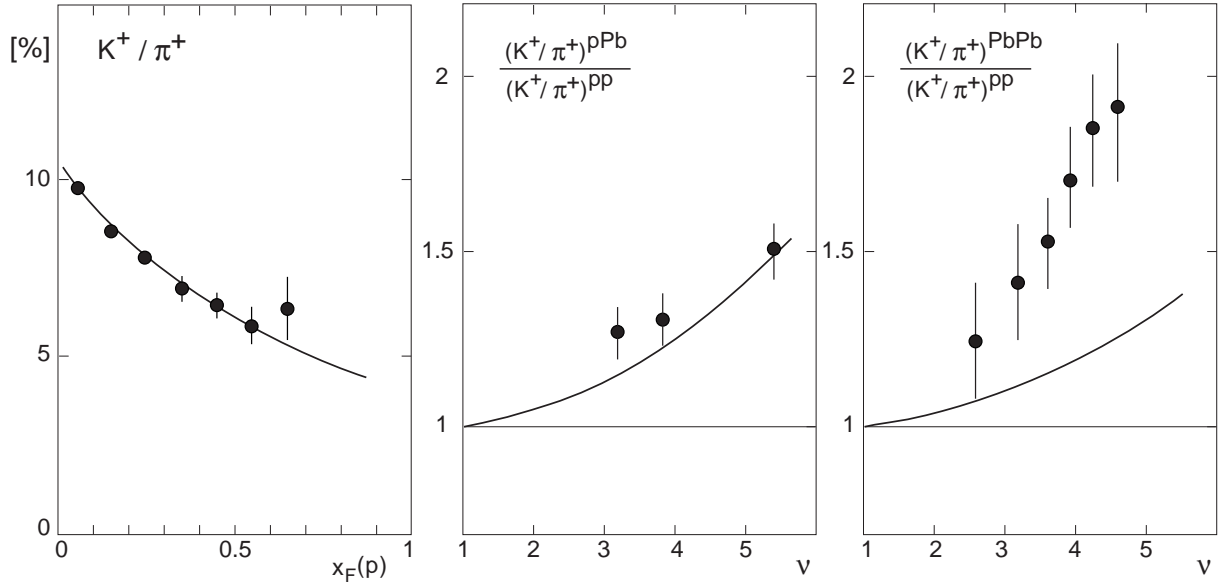
Figure 8: a) Dependence of K^+/\pi^+ ratio in the forward hemisphere of p+p collisions on x_F(p) of final state baryon; b) prediction (solid line) and measurement of forward K^+/\pi^+ ratio in p+Pb collisions as function of \nu , normalized to p+p; c) prediction (solid line) and measurement of forward K^+/\pi^+ ratio in Pb+Pb collisions as function of \nu , normalized to p+p.
