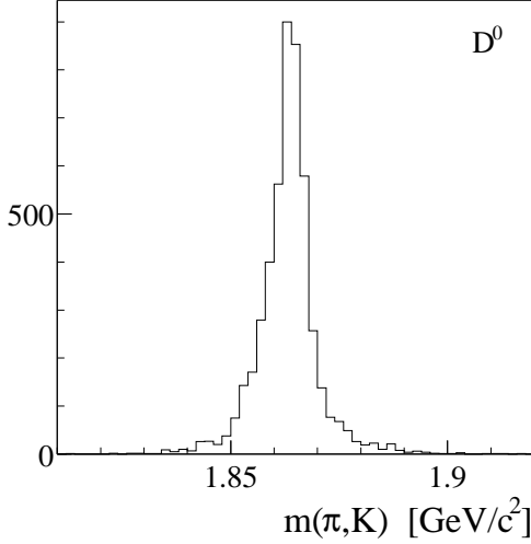
Figure 1: The invariant mass spectrum of pairs of kaons and pions, obtained from the simulation of 10000 D^0 decays.
