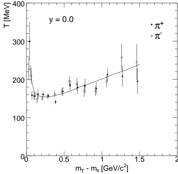
Figure 23: Local slope of the m_T distribution as a function of m_T - m_\pi for \pi^+ and \pi^- . The line shown is to guide the eye
