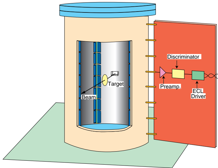
Figure 2: The grey proton detector
