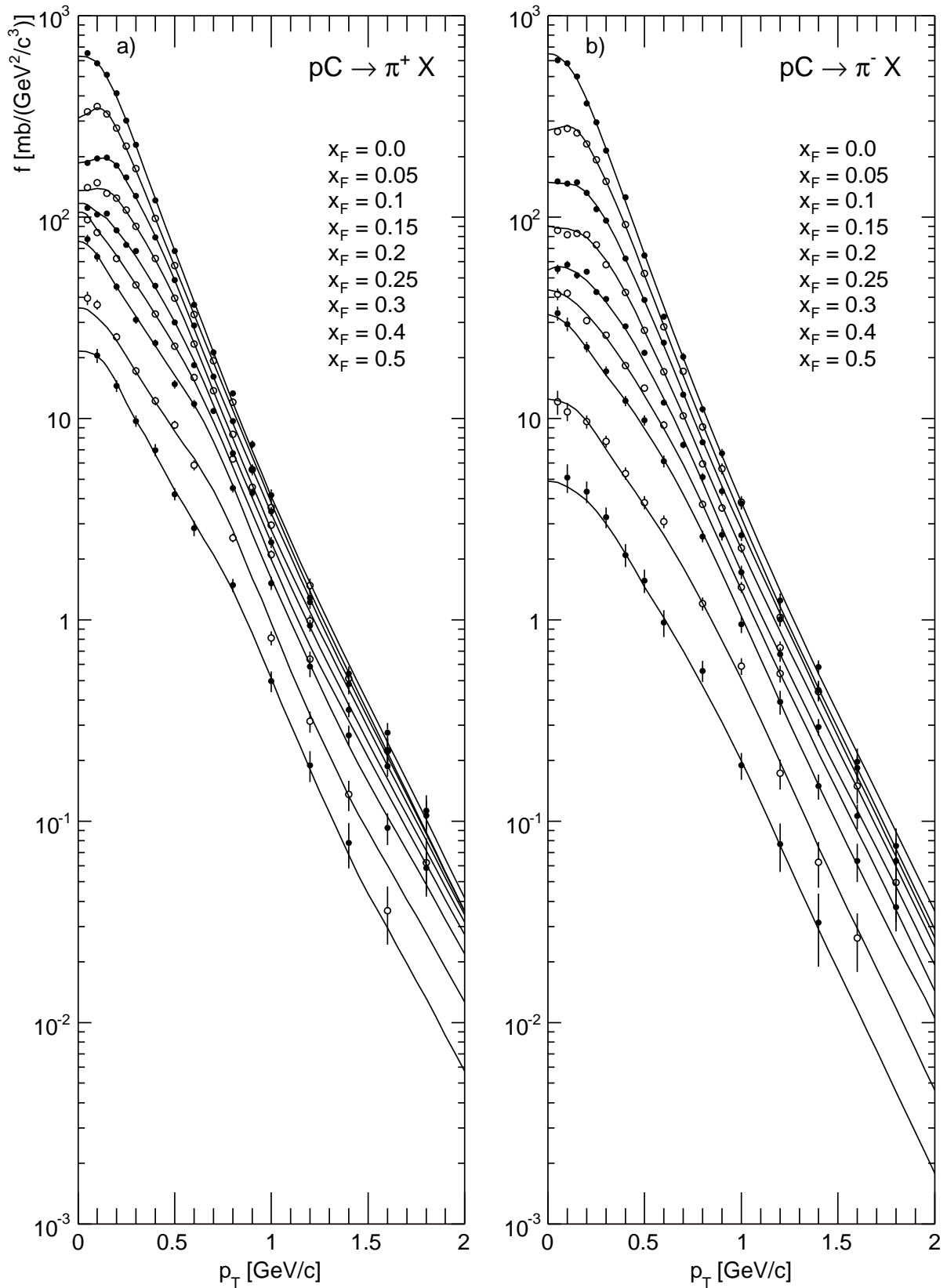
Figure 17: Invariant cross section as a function of p_T at fixed x_F for a) \pi^+ and b) \pi^- produced in p+C collisions at 158 GeV/c. The x_F values given in the Figure are to be correlated to the respective distributions in decreasing order of cross section
