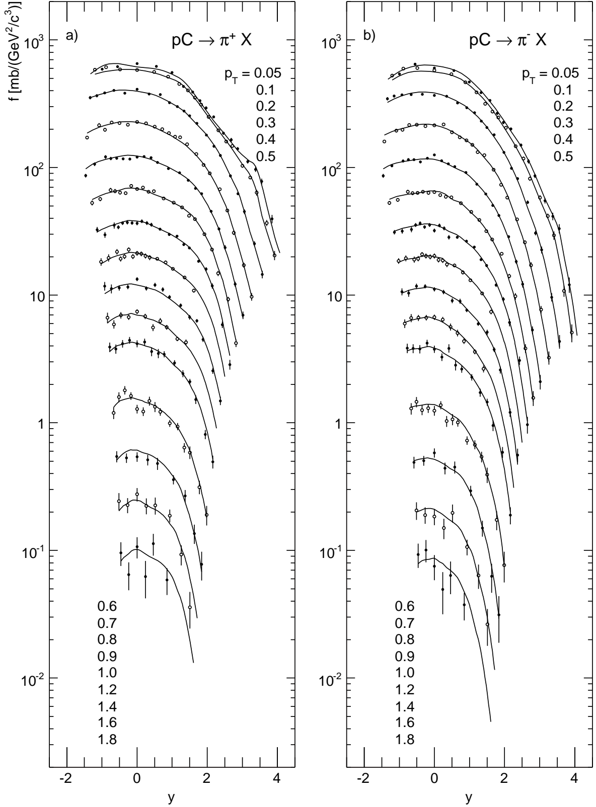
Figure 21: Invariant cross section as a function of y at fixed p_T for a) \pi^+ and b) \pi^- produced in p+C collisions at 158 GeV/c. The p_T values given in the Figure are to be correlated to the respective distributions in decreasing order of cross section
