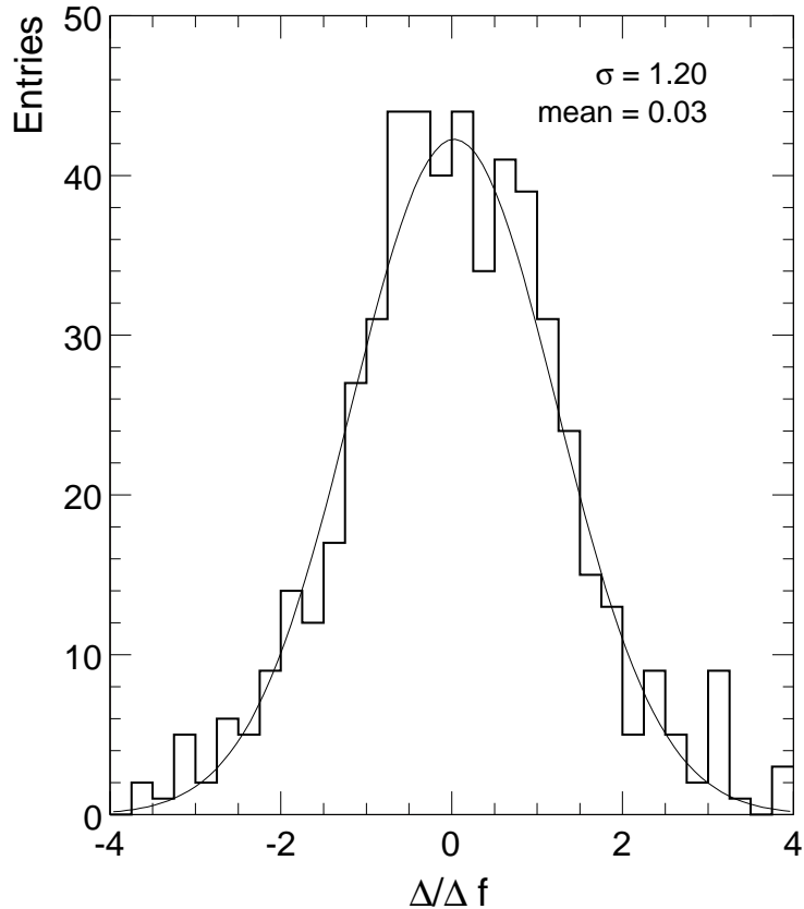
Figure 16: Histogram of the differences \Delta between the measured invariant cross sections and the corresponding interpolated values ( \pi^+ and \pi^- combined) divided by the experimental uncertainty \Delta f of the data points
