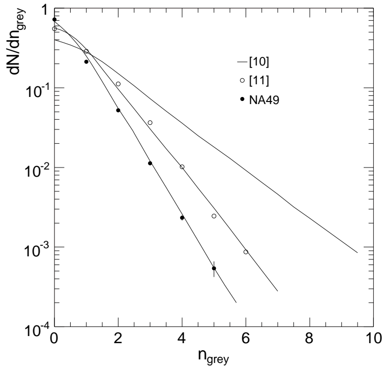
Figure 3: Number of grey protons n_{\text{grey}} distribution. The lines through the data points refer to the acceptances of 60% and 45% for [11] and NA49, respectively, as obtained from the prediction [10]
