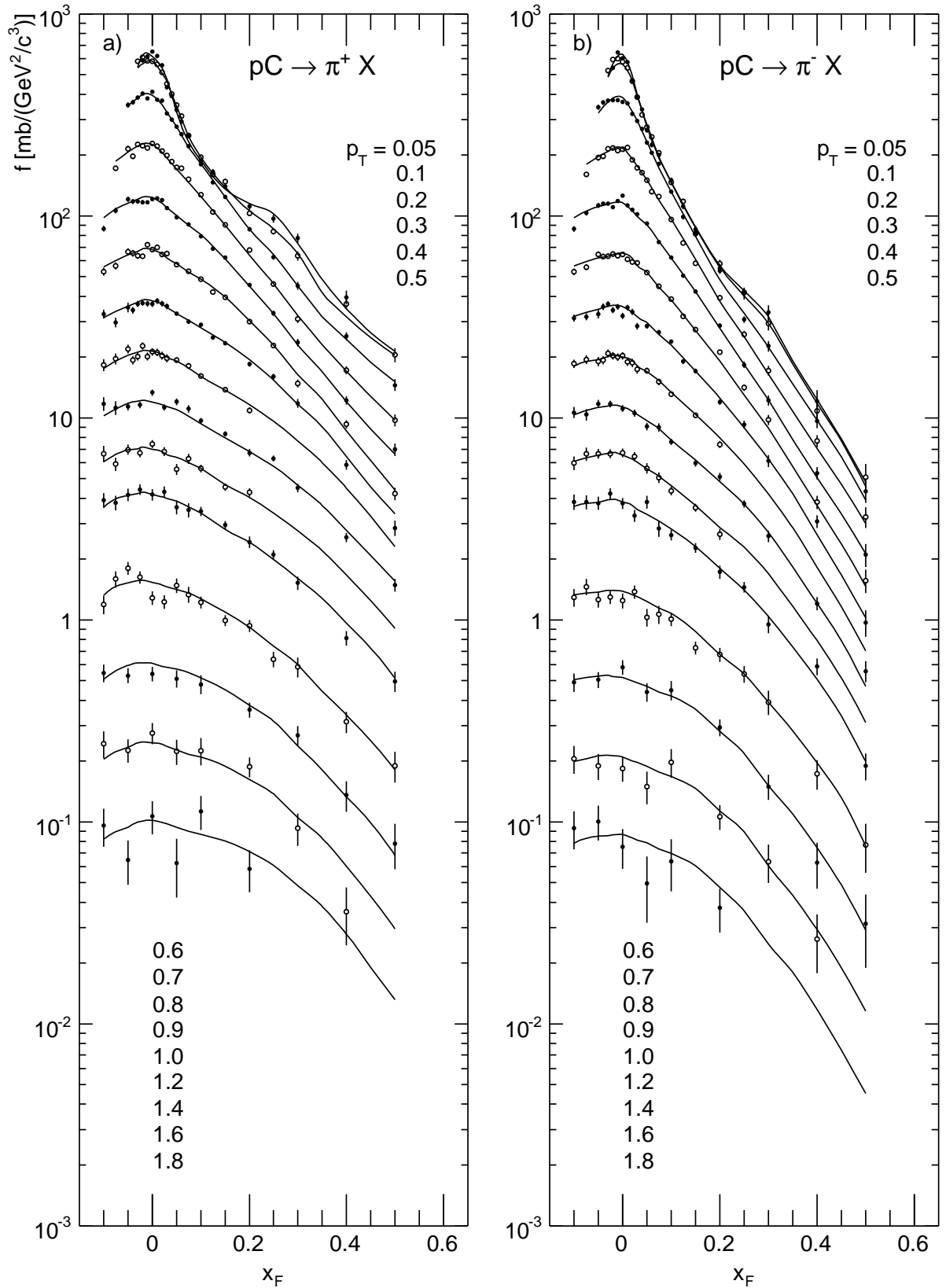
Figure 18: Invariant cross section as a function of x_F at fixed p_T for a) \pi^+ and b) \pi^- produced in p+C collisions at 158 GeV/c. The p_T values given in the Figure are to be correlated to the respective distributions in decreasing order of cross section
