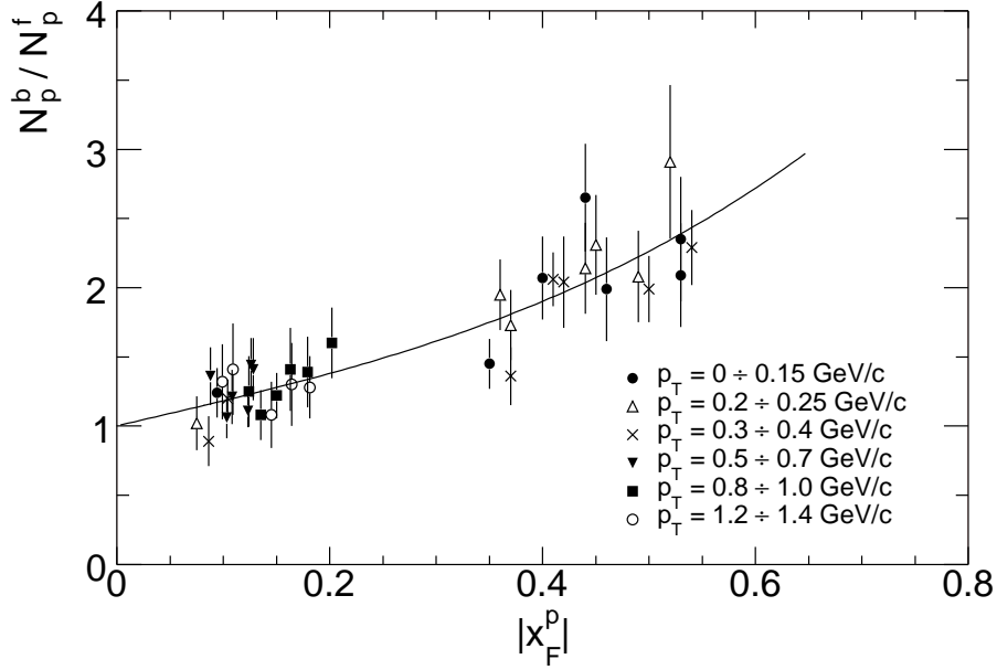
Figure 8: Backward/forward yield ratio for protons
