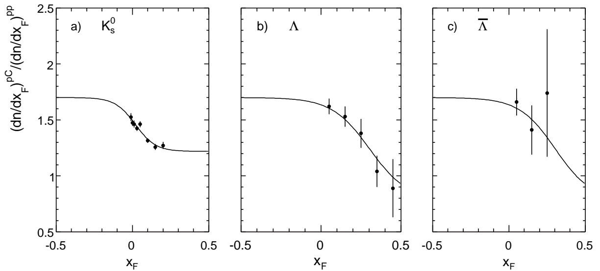
Figure 12: Yield ratios for a) K_S^0 , b) \Lambda and c) \bar{\Lambda}
