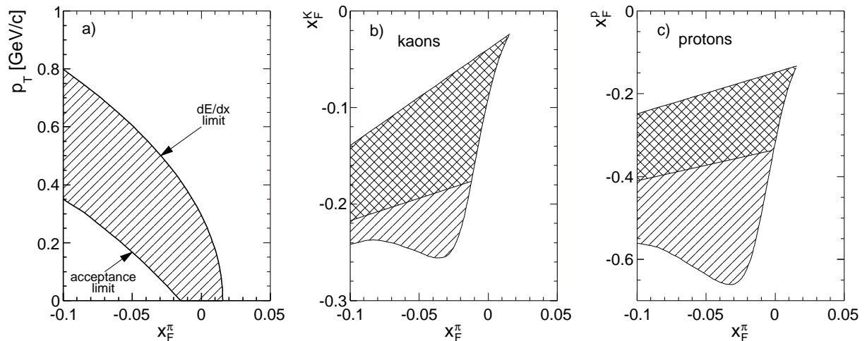
Figure 7: dE/dx cross-over region: a) in (x_F, p_T) plane of the pions, b) in (x_F^\pi, x_F^K) plane, and c) in (x_F^\pi, x_F^p) plane. The single hatched areas in b) and c) correspond to the regions where pions can be identified due to the 1/\beta^2 increase of energy loss of the kaons and protons, respectively
