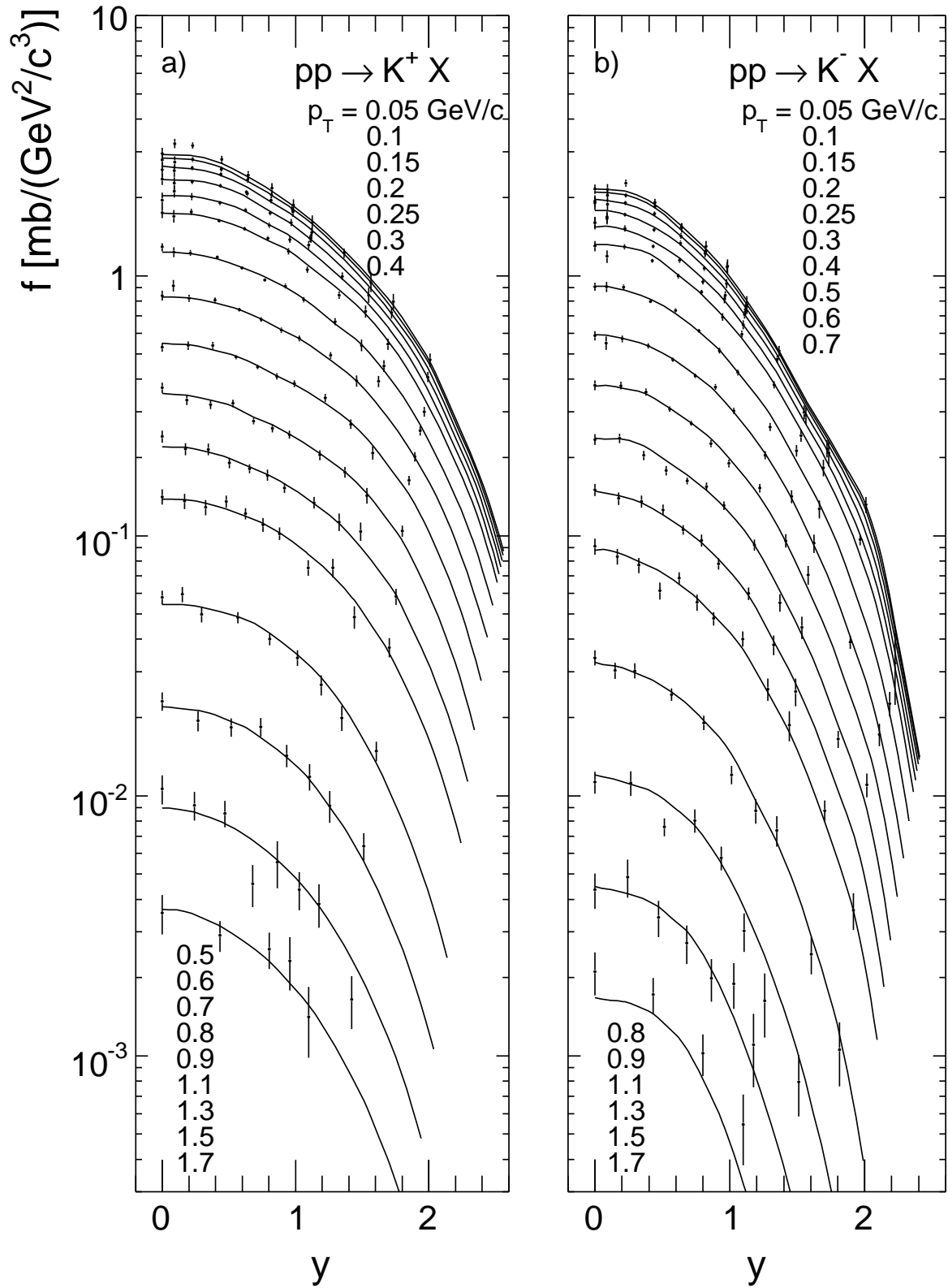
Figure 23: Double differential invariant cross section f(x_F, p_T) [mb/(GeV 2 /c 3 )] as a function of y at fixed p_T for a) K + and b) K - produced in p+p collisions at 158 GeV/c beam momentum. The lines show the result of the data interpolation, Sect. 6.2
