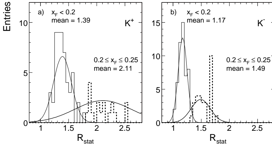
Figure 12: R_{\text{stat}} = \sigma_{\text{stat}}/(1/\sqrt{N}) for the bins x_F < 0.2 (solid line) and 0.2 \leq x_F \leq 0.25 (dashed line); a) K^+ and b) K^-
