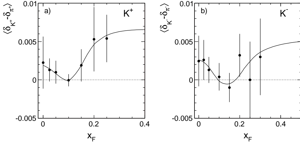
Figure 8: Mean deviations in units of minimum ionization of a) K^+ and b) K^- with respect to the pion position \langle \delta_{K^\pm} - \delta_\pi \rangle as a function of x_F , averaged over p_T
