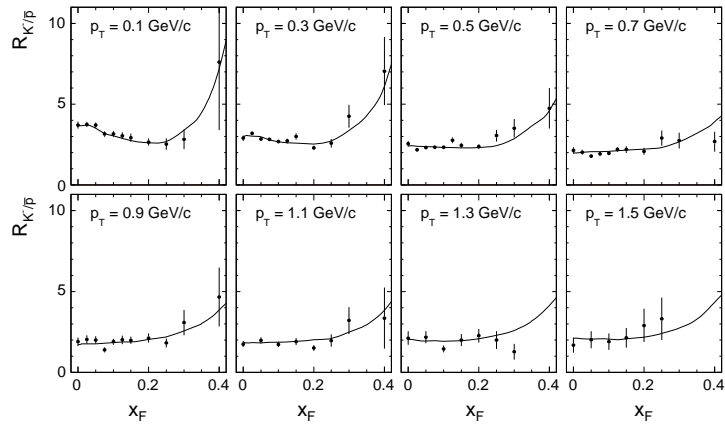
Figure 40: R_{K-\bar{p}} as a function of x_F at fixed p_T . The lines show the result of the data interpolation, Sect. 6.2
