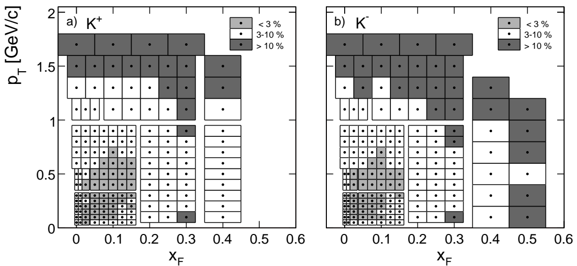
Figure 4: Binning schemes in x_F and p_T for a) K + and b) K - together with information on the statistical errors
