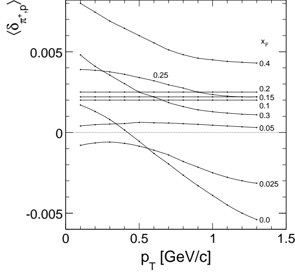
Figure 7: Mean deviation \langle \delta_{\pi^+,p} \rangle , in units of minimum ionization, of \pi^+ and proton dE/dx with respect to the Bethe-Bloch parametrization as a function of p_T for different values of x_F
